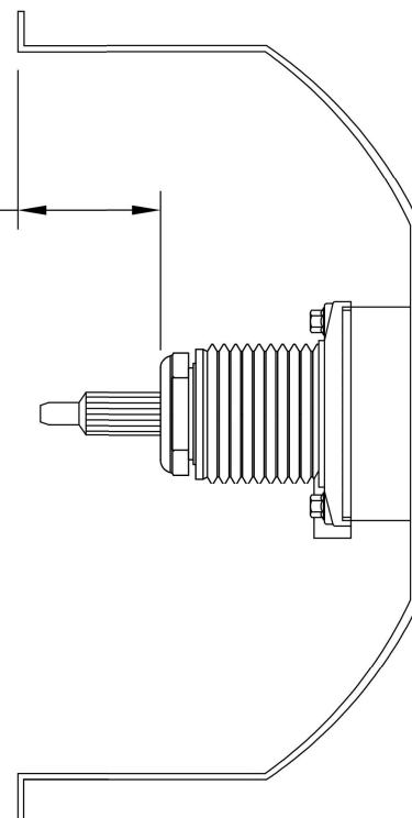
BELLHOUSING SIDE VIEW CUT-A-WAY
